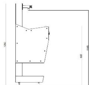
SIDE ELEVATION
